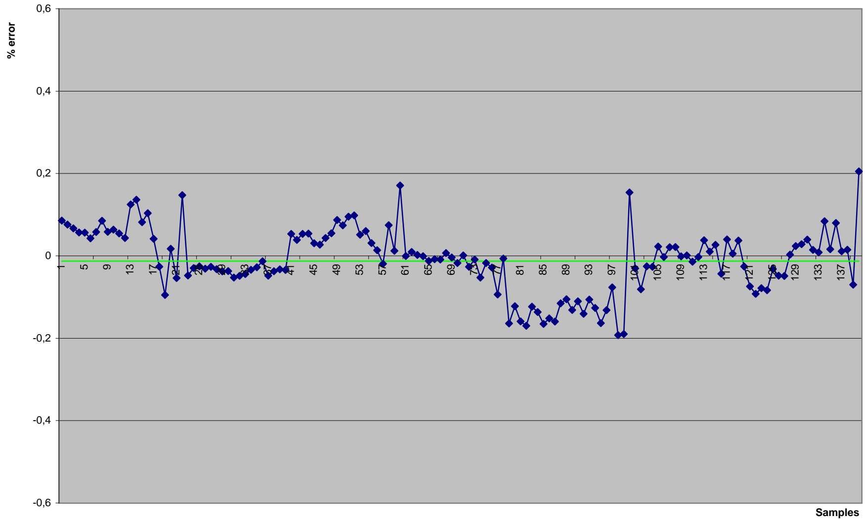
MMD5 Dispenser - % error over 140 sample of 20 measurements - (Average Error -0,01251%)
